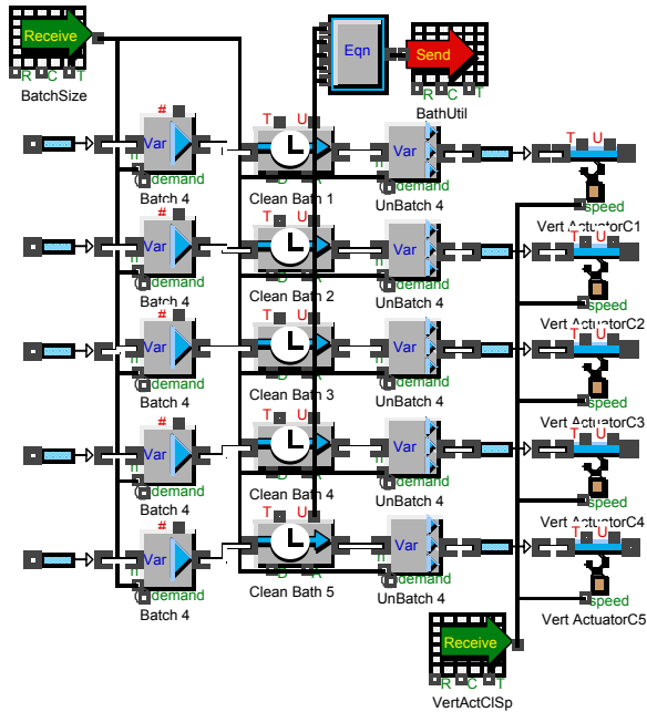
Figure 2. Clean Bath Process Group
