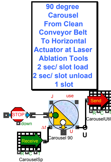
Figure 4. 90-Degree Carousel
