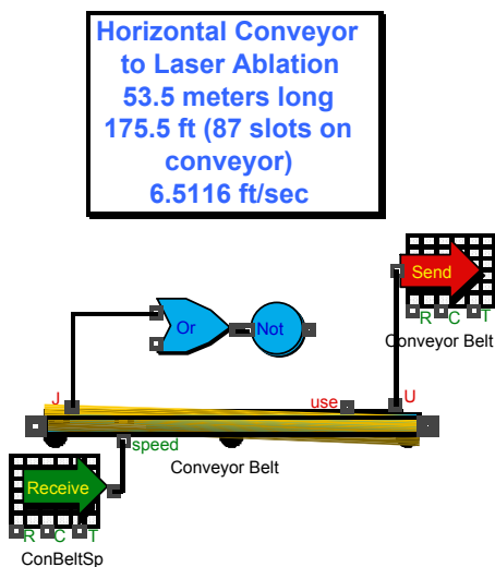
Figure 3. Horizontal Conveyor
